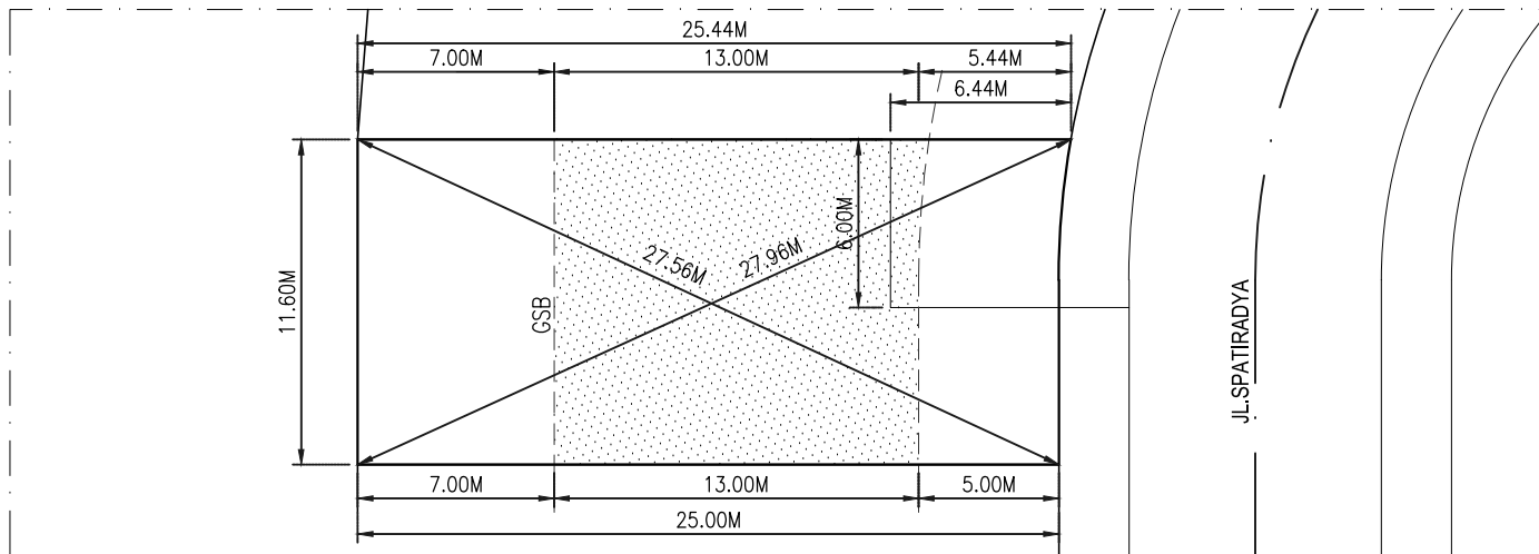
DENAH UNIT HUNIAN JL.SPATIRADYA NO. 26 SKALA 1 : 300
